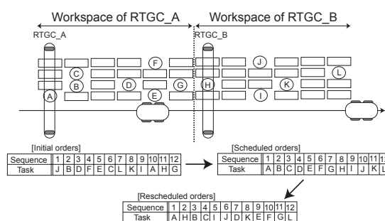
Fig.2 Example of Container Storage Scheduling
