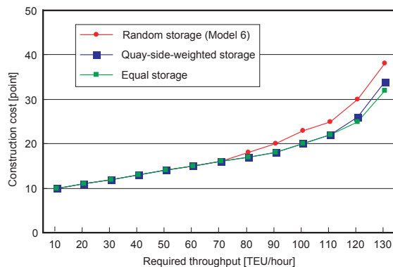
Fig.5 Comparison Results of the Total Construction Costs Under the all Transportation Rules
