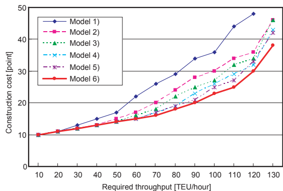
Fig.4 Comparison Results of the Total Construction Costs Under the Random Container Transportation
